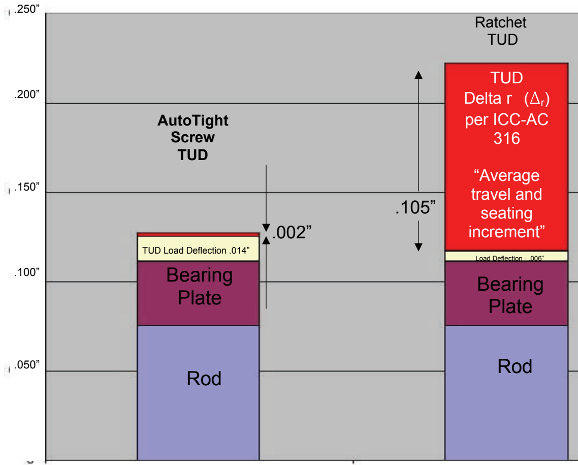
Comparison of System Deflection—Variable - Shrinkage Compensator Type
